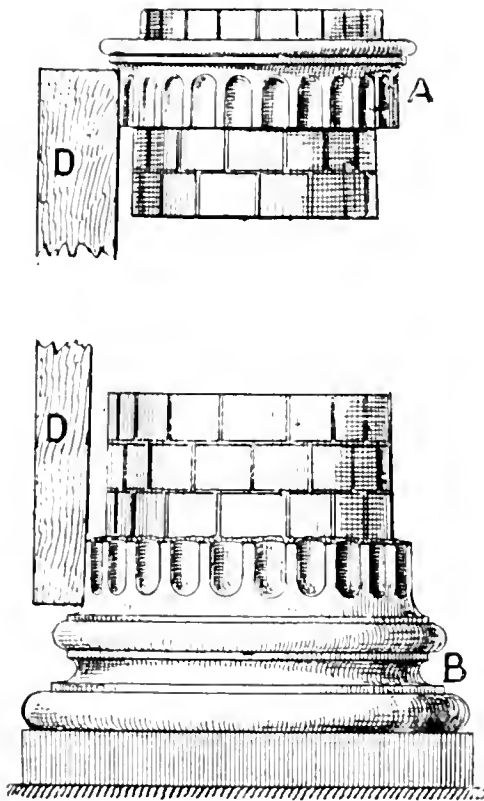
NO. 31.—FLOATED FLUTED COLUMNS— RIM METHOD.
